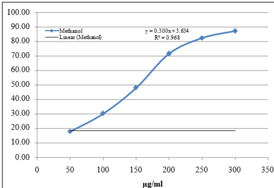
Fig 1: Average percentage cell inhibition of methanolic leaf extract of M. oleifera against A549 cells
