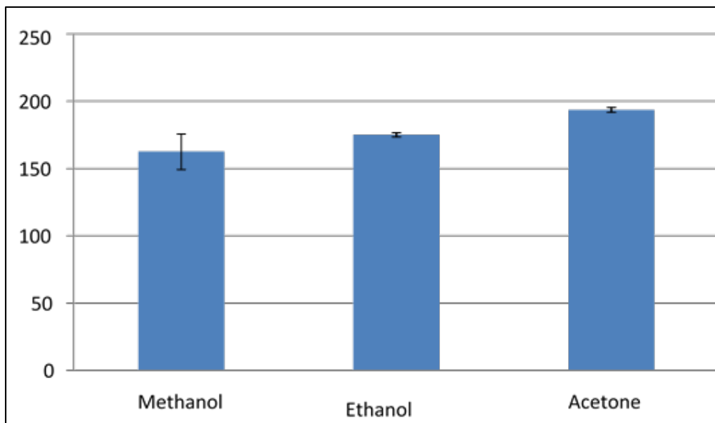
Fig 4: Fifty percent inhibition ( \text{IC}_{50} ) concentration of M. oleifera crude extract with different solvents for A549 cells
